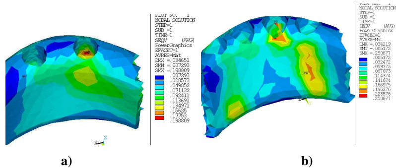
Figure 5: von Mises stresses in the trabecular bone of a 'normal' mandible: a) 'traditional' implant support design, b) 'modified' implant support design. Stress values are in MPa.
